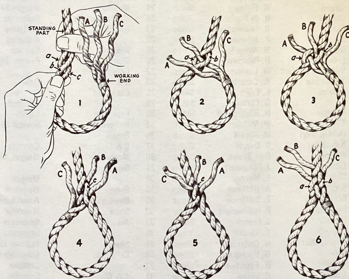
The Eye Splice
